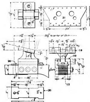
Figs. 1568-1574. Expansion Pad, Clamps and Plate for Ten-Wheel (4-6-0) Locomotive. P. R. R.
